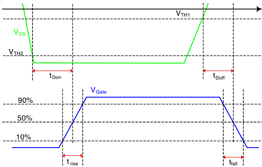
Fig. 15 - Timing Diagrams
